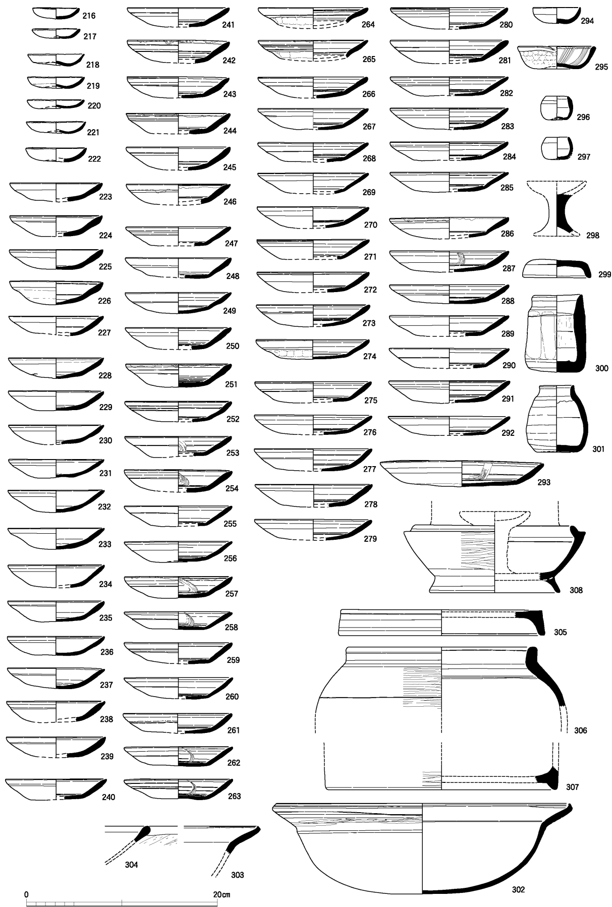
图16 东区SK51下段出土土器实测图1 (1:4)
