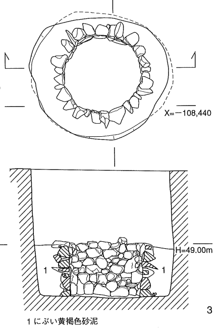
⊙ A区井戸A354 Y=-21,160
