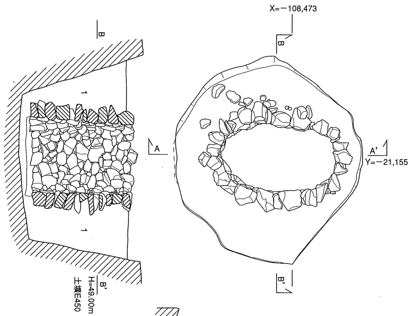
● E区石組土塙 E 22
