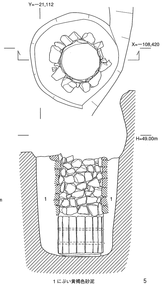
③ C区井戸C1192
