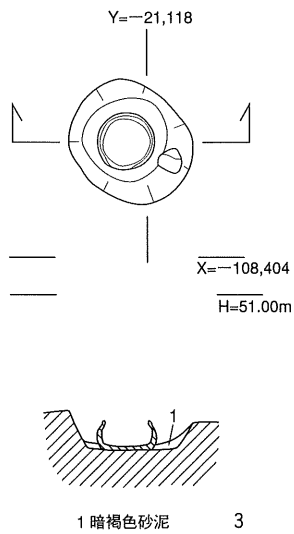
④ C区埋納土壙C494
