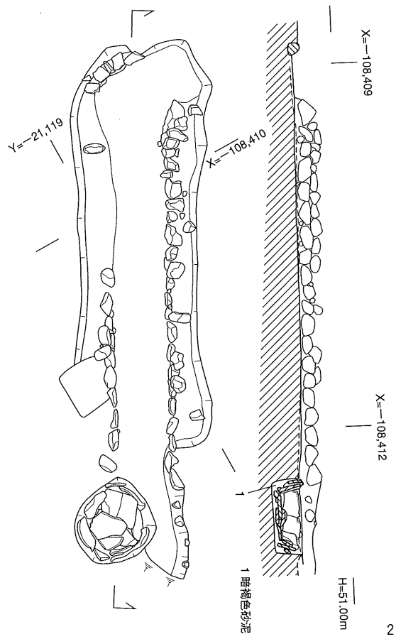
② C区溝C113・瓦組柵C153
