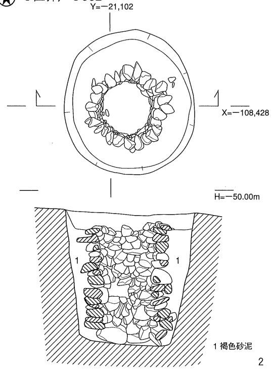
③ C区井戸C1192
